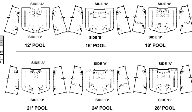
HOLE CHART FOR 6" STANDARD & 6-1/2" RESIN FLARE TOP RAIL POOLS
