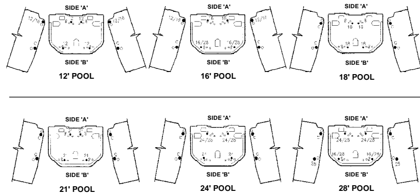
HOLE CHART FOR 8" RESIN & 8-1/2" STEEL TOP RAIL POOLS
